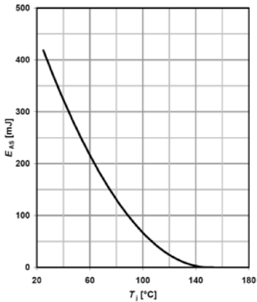
Avalanche energy
