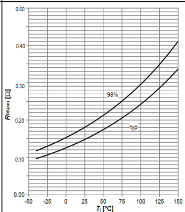
Diagram 8: Drain-source on-state resistance
