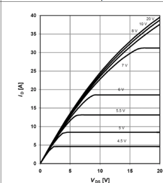
Typ. output characteristics T_J = 125^\circ\text{C}
