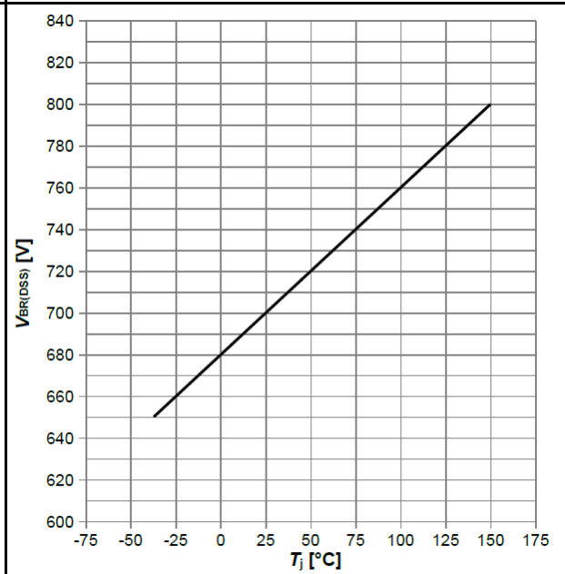
Diagram 13: Drain-source breakdown voltage
