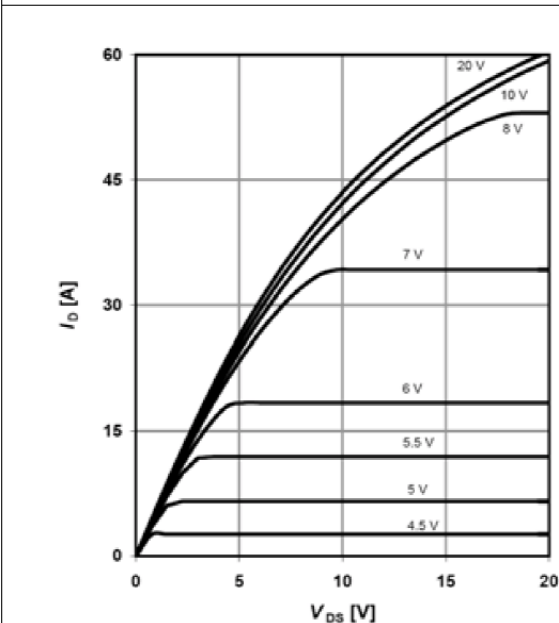
Typ. output characteristics T_c = 25^\circ\text{C}
