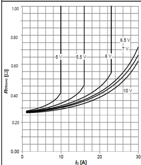
Diagram 7: Typ. drain-source on-state resistance
