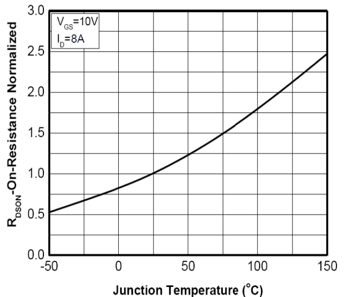
Normalized on resistance vs temperature
