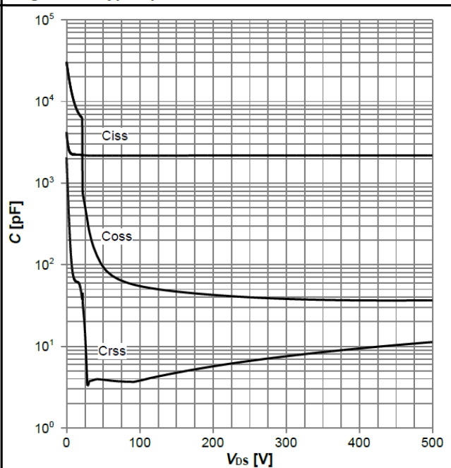
Diagram 14: Typ. capacitances
