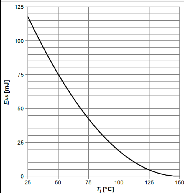
Diagram 12: Avalanche energy
