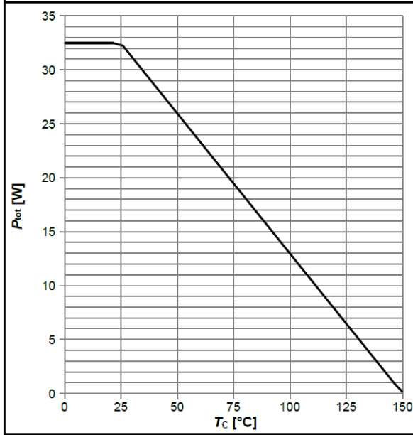
Diagram 1: Power dissipation
