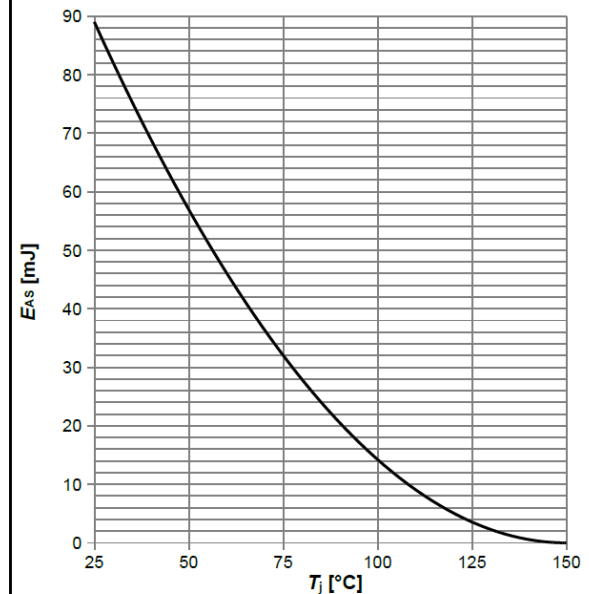
Diagram 12: Avalanche energy
