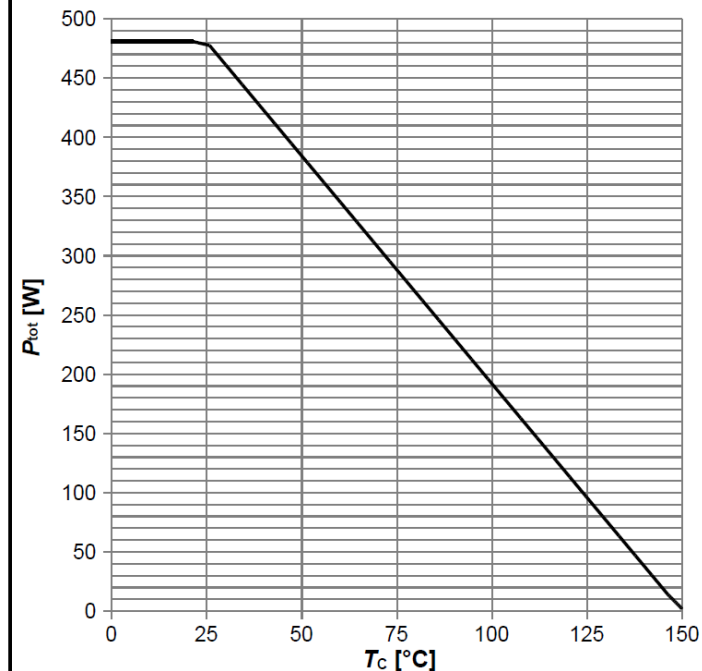
Diagram 1: Power dissipation
