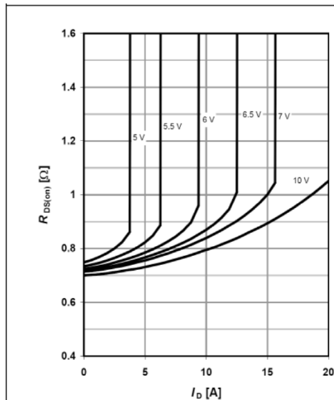
Typ. drain-source on-state resistance
