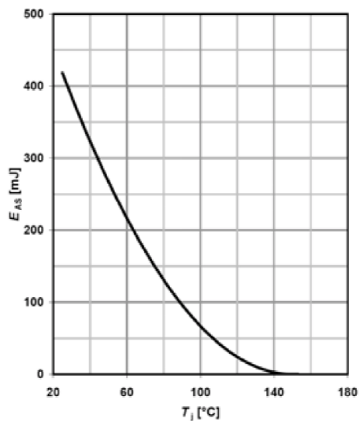
Avalanche energy
