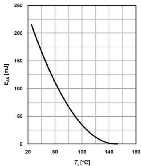
Avalanche energy
