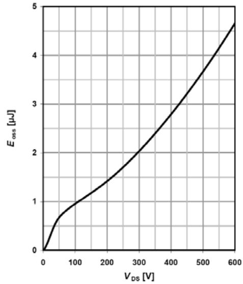
Typ. E_{oss} stored energy
